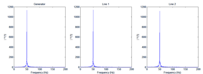
Figure 1.8: Frequency Spectrum of Voltage
