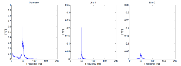
Figure 1.7: Frequency Spectrum of Current
