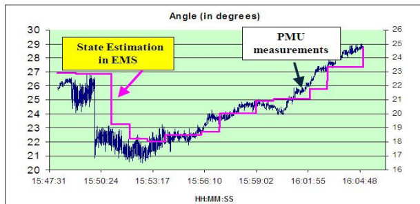
Figure 1.2: State estimation v.s. PMU measurements [10]
