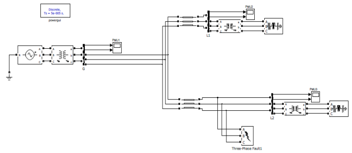
Figure 1.5: Wide Area SIMULINK Model
