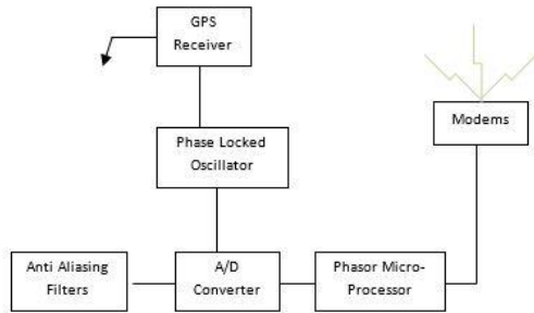
Figure 1.1: Phasor Measurement Diagram Unit Block If enough PMUs can be installed across a large power transmission network, the real time system operating condition can be directly measured by PMUs. In addition, as the PMUs have a high data reporting rate, the system dynamics can be captured when the system is subjected to disturbances.
