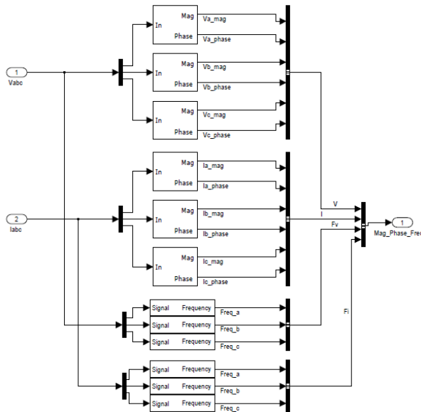
Figure 1.4: Phasor Measurement Unit MATLAB Model
