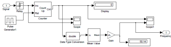
Figure 1.3: Frequency Measurement Unit SIMULINK Model
