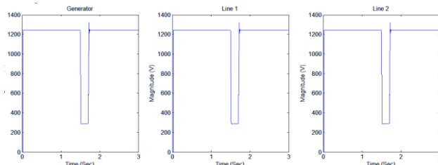
Figure 1.10: Line Voltage
